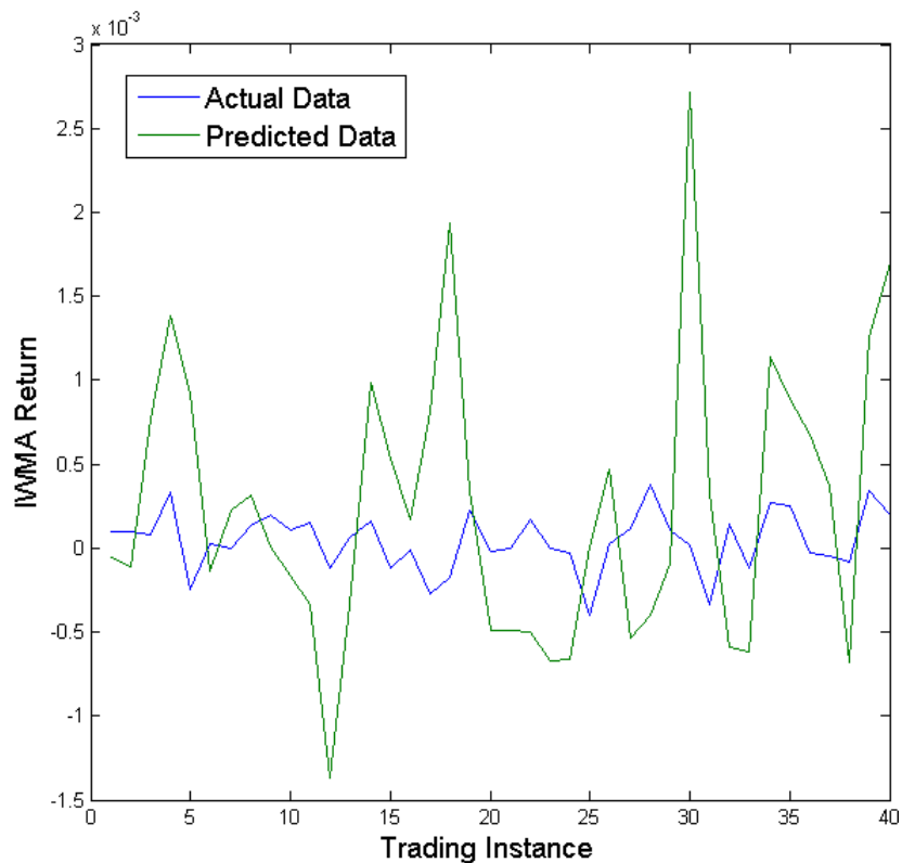
Figure 15: Monte Carlo Simulation
